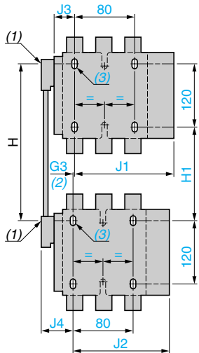
Assembly A
