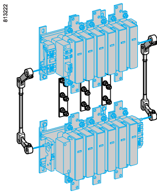
LA9 FX971
