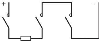
3 poles
