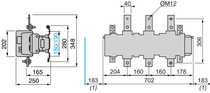
LC1 F78040
