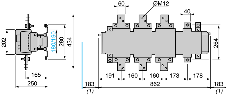
LC1 F78040
